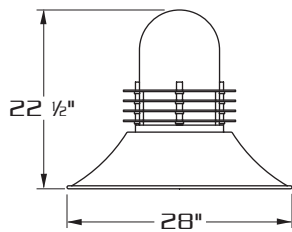
DSCPM25 [250 W. MAX.]
